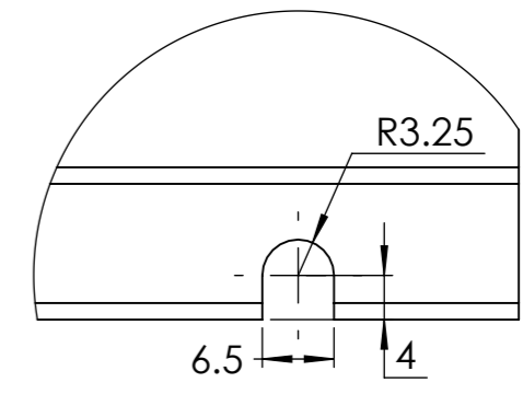
DETAIL A SCALE 2 : 1.5
